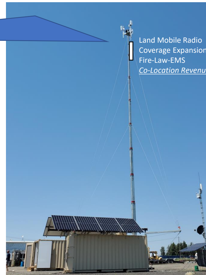
Self-Contained Site w/Off Grid Power
